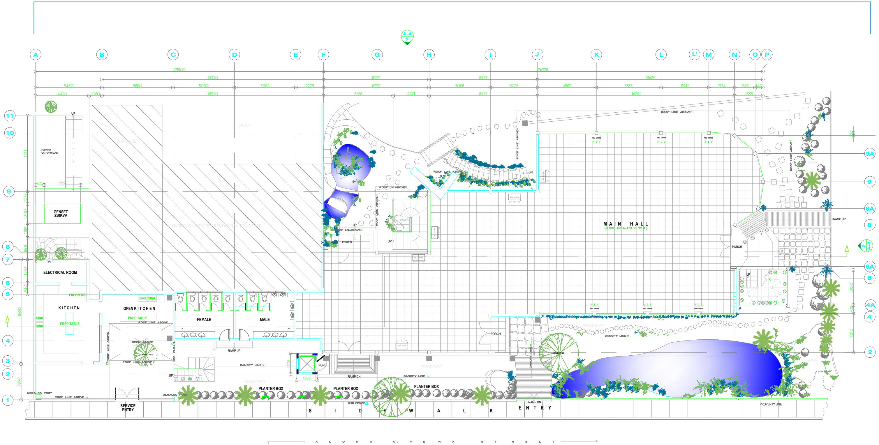
1 A-4 GROUND FLOOR PLAN SCALE: 1:100 MTS
